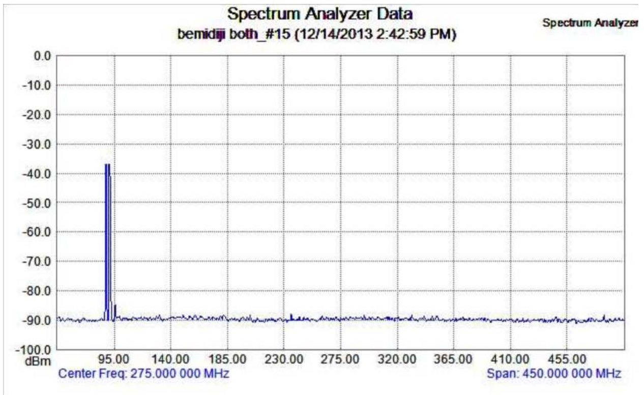
Measurement of both stations with a span of 50 MHz to 500 MHz. The bandwidth was set to 1 kHz.
