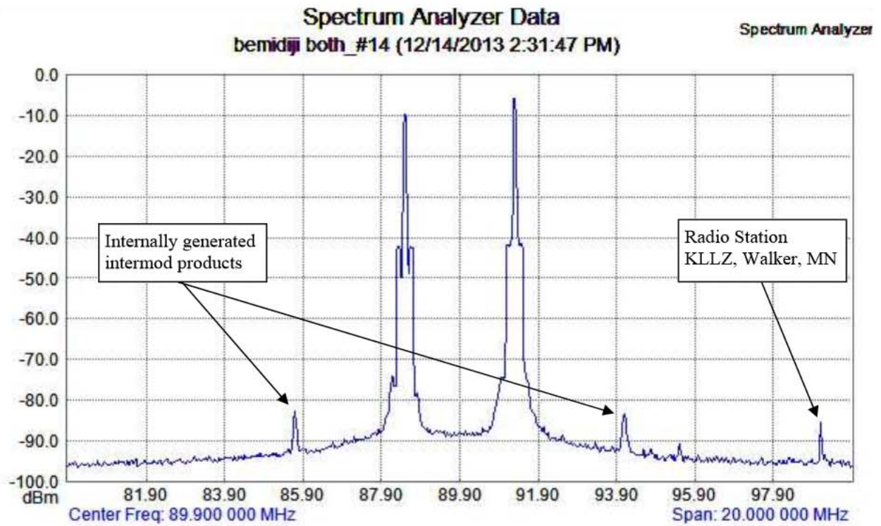
Measurement of both stations with the span set to 20 MHz. The bandwidth was set to 300 Hz.
