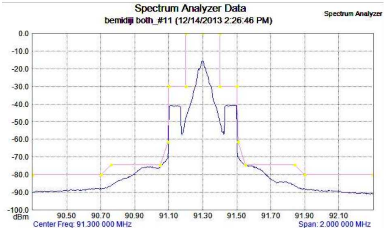
Results of the measurement of KNBJ FM and HD.
